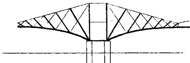
Fig. 470. A two-armed cantilever of the Forth Bridge. Thick lines, compression-members (bones); thin lines, tension-members (ligaments).
