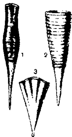
Fig. 409. Pteropod shells:
