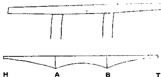
Fig. 477. Two-armed cantilever and its stress diagram.
